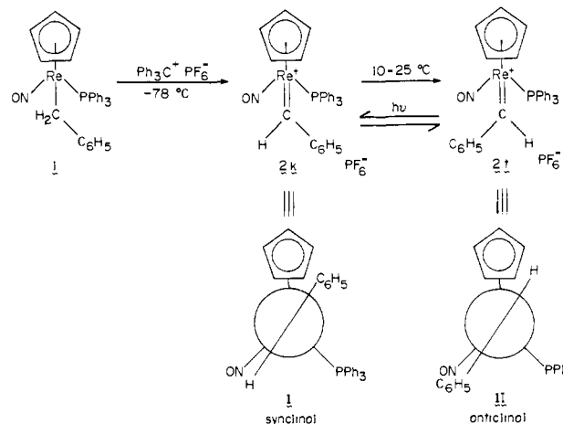
Scheme I. Syntheses and Interconversions of Isomeric Benzylidene Complexes 10
