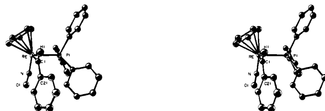
Figure 2. Stereoview of the molecular structure of ac\text{-}[(\eta\text{-C}_5\text{H}_5)\text{Re}(\text{NO})(\text{PPh}_3)(=\text{CHC}_6\text{H}_5)]^+\text{PF}_6^-\cdot\text{CHCl}_3 ( 2t · \text{CHCl}_3 ).
