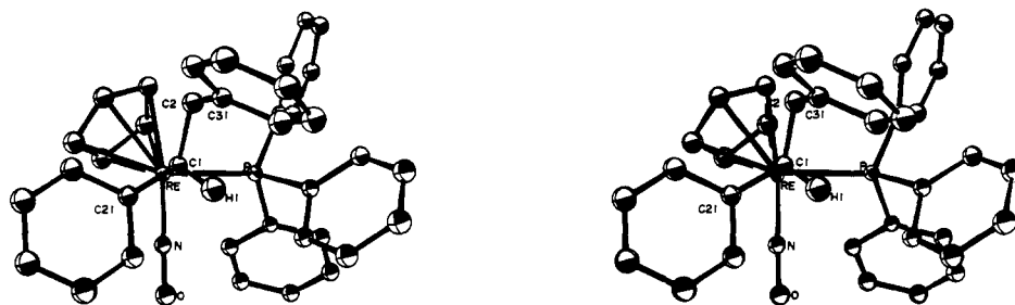
Figure 4. Stereoview of the molecular structure of (SS,RR)-(\eta-C_5H_5)Re(NO)(PPh_3)(CH(CH_2C_6H_5)C_6H_5)\cdot CH_2Cl_2 ( 5t · CH_2Cl_2 ).
