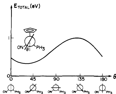
Figure 1. Calculated E_{\text{total}} for [(\eta\text{-C}_5\text{H}_5)\text{Re}(\text{NO})(\text{PH}_3)(=\text{CH}_2)]^+ as the =\text{CH}_2 ligand is rotated.
