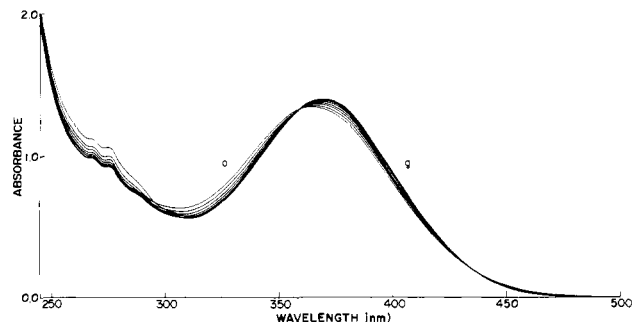
Figure 3. Absorption spectra recorded as a (55 \pm 3):(45 \pm 3) 2\mathbf{t}/2\mathbf{k} mixture in \text{CH}_2\text{Cl}_2 (prepared by photolysis at -78 °C) was warmed to room temperature: initial spectrum, trace a; final spectrum, trace g.
