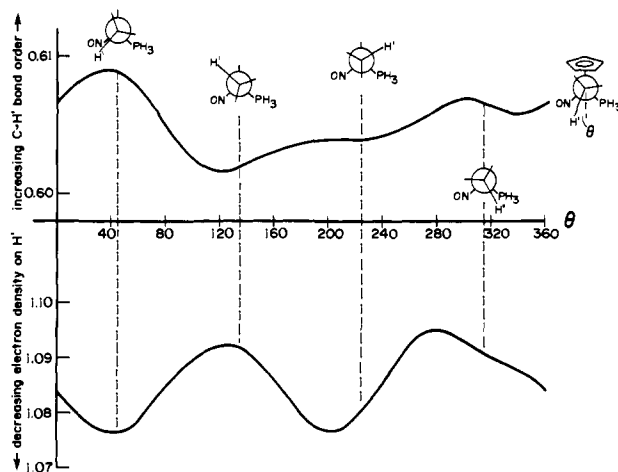
Figure 6. Calculated change in C-H' bond order and electron density on H' as the Re-C \sigma bond in (\eta\text{-C}_5\text{H}_5)\text{Re}(\text{NO})(\text{PPh}_3)(\text{CH}_2\text{H}') is rotated through 360° (C-H' = bond arbitrarily elongated to 1.4 Å).
